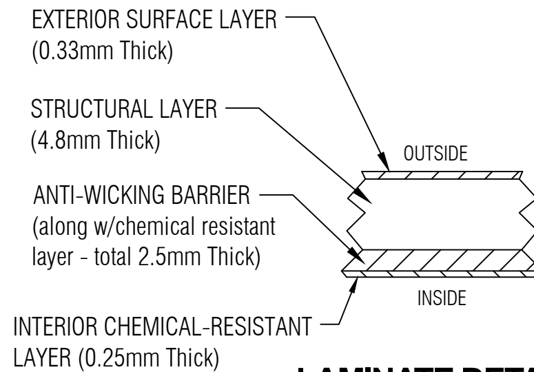
LAMINATE DETAIL 1 N T S
