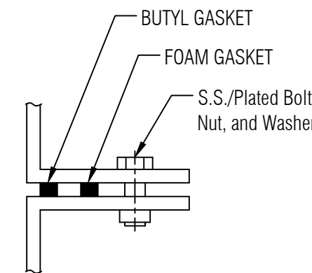
FLANGE TO FLANGE CONNECTION DETAIL 2 N T S
