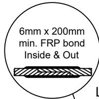
SECTION-JOINT DETAIL
