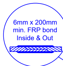
SECTION-JOINT DETAIL
