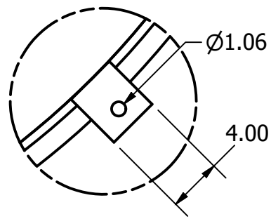
LIFTING LUG DETAIL A SCALE 1/10
