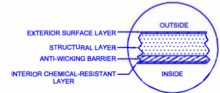
LAMINATE DETAIL
