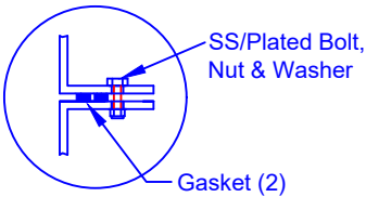
FLANGE CONNECTION DETAIL
