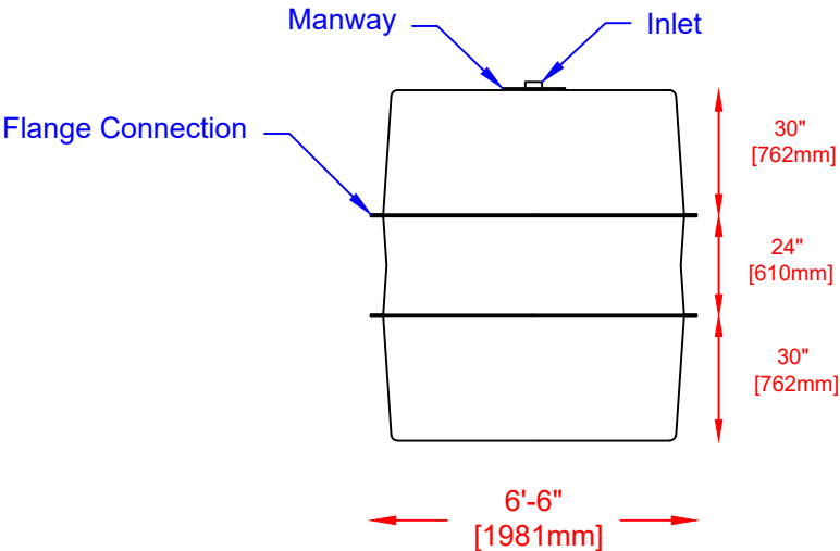
END VIEW
