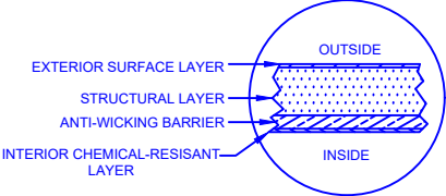
LAMINATE DETAIL
