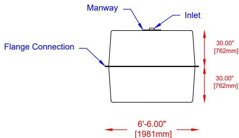
END VIEW
