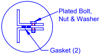
FLANGE CONNECTION DETAIL
