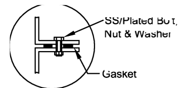
FLANGE CONNECTION DETAIL
