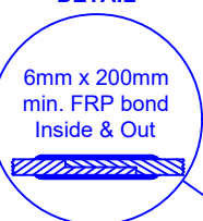
SECTION-JOINT DETAIL
