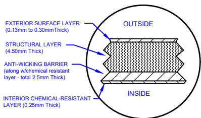
LAMINATE DETAIL
