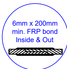
SECTION-JOINT DETAIL
