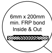
SECTION-JOINT DETAIL
