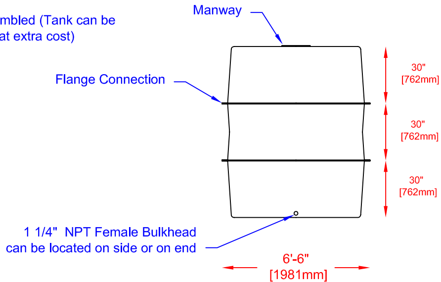
END VIEW
