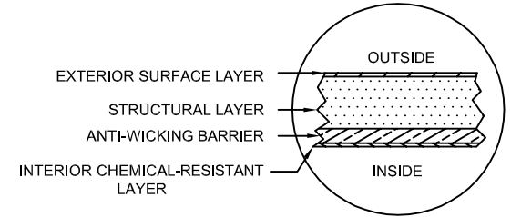
LAMINATE DETAIL
