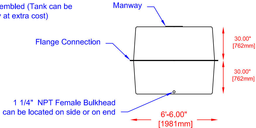
END VIEW
