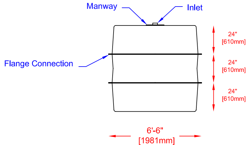
END VIEW
